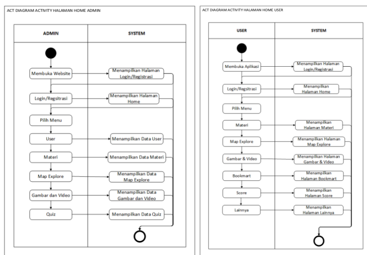
Gambar 2. Activity Diagram Halaman Home Admin dan User
