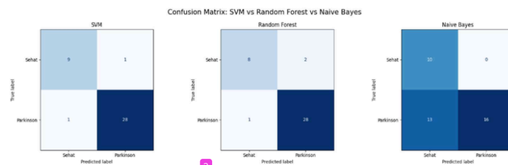
Figure 3. Confusion Matrix Comparison
