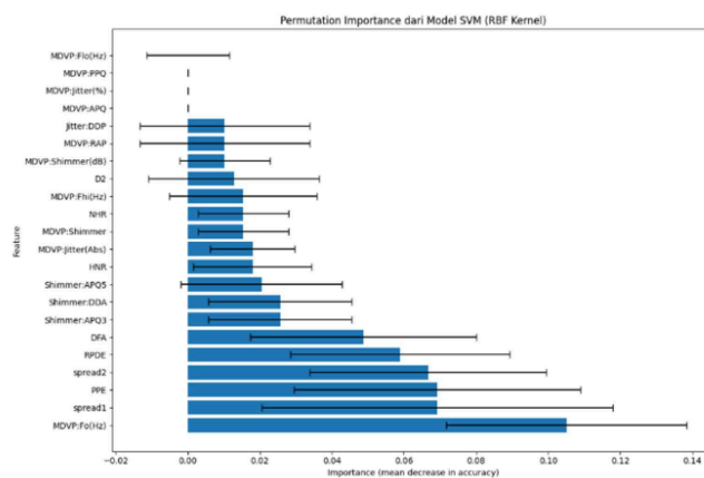
Figure 4. Permutation Importance Visualization
