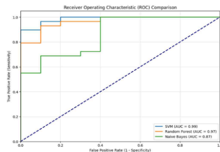
Figure 2. ROC Curve Comparison
