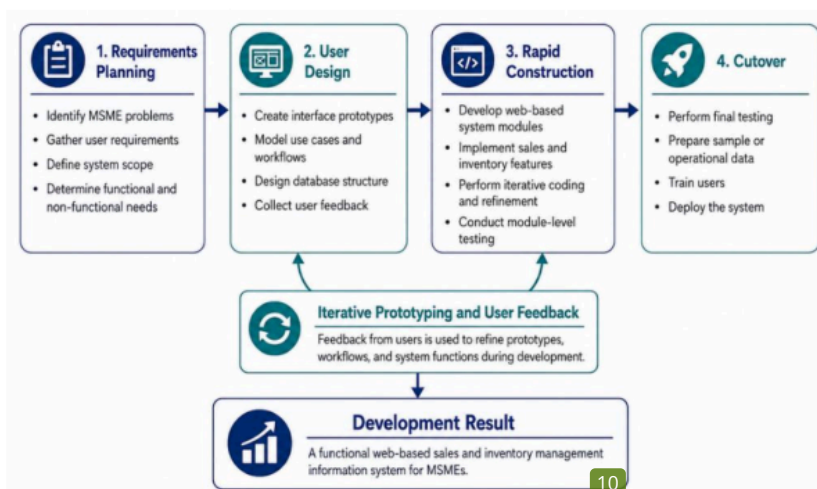
Figure 2. Rapid Application Development stages used in the development of the web-based sales and inventory management system
